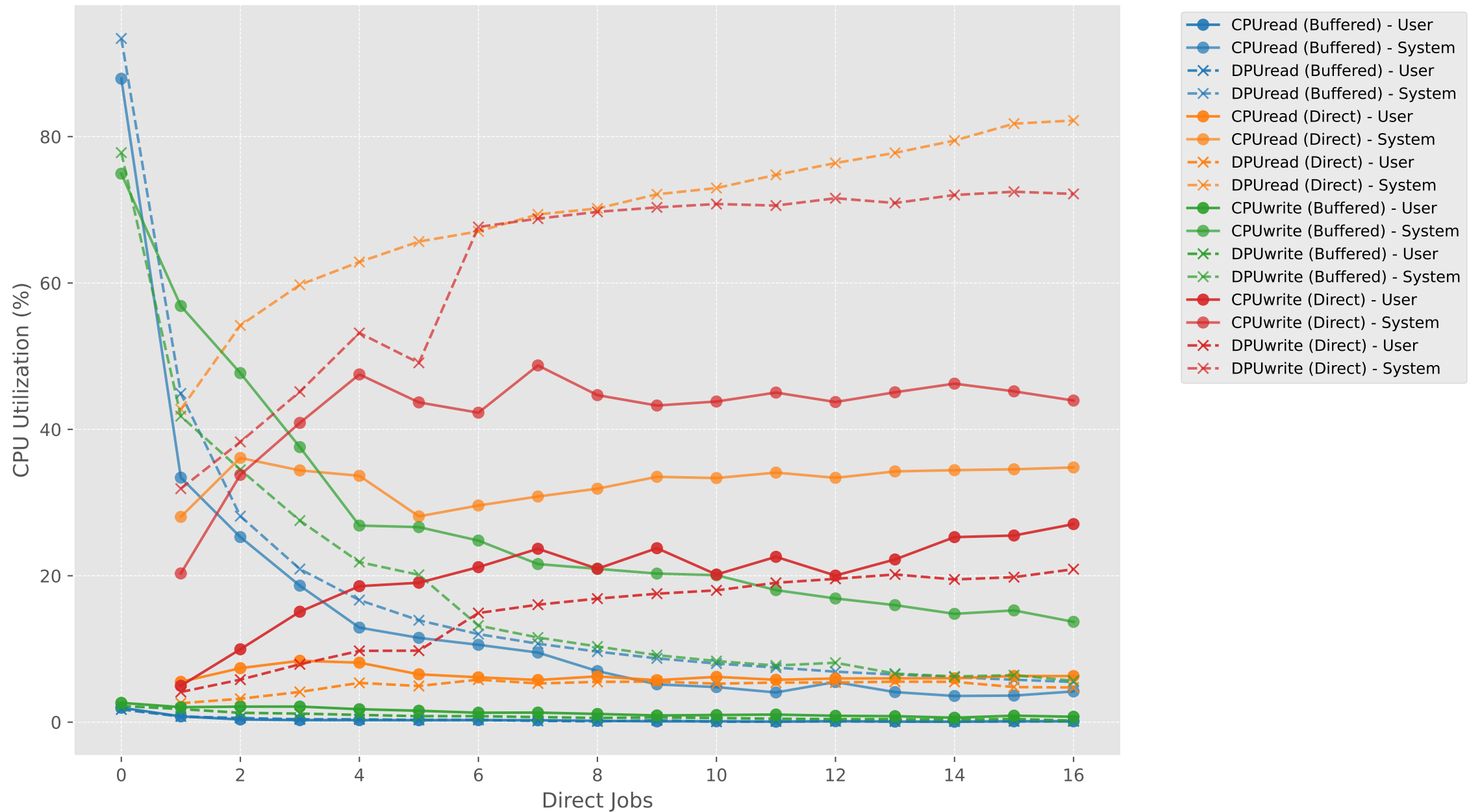
CPU Utilization vs Direct Jobs (buffered1_directN) - SEQ (CPU vs DPU)
